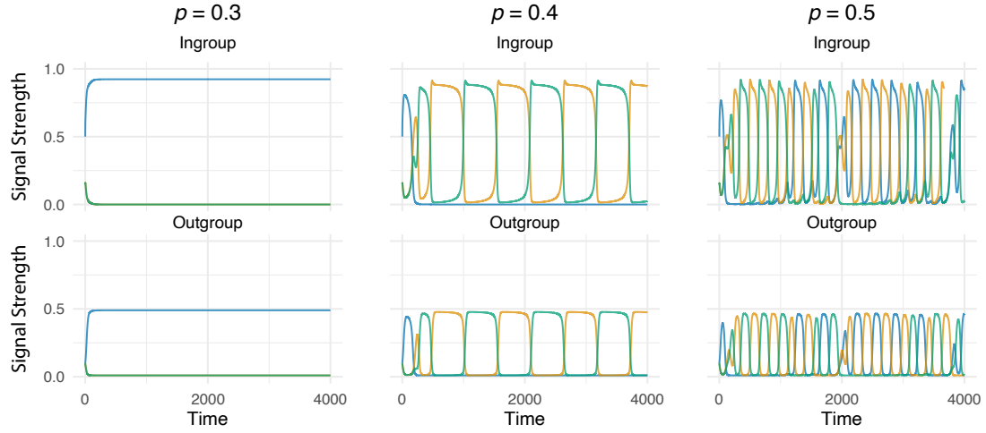
FIGURE A1. Example dynamics for ingroup signal strengths (top) and outgroup signal awareness (bottom) for different values of punishment, p . Here c = 1 .
