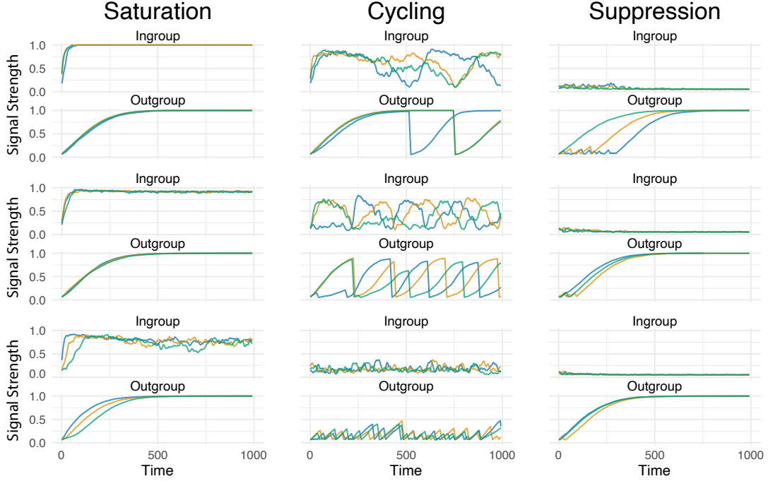
FIGURE 3. The three classes of model dynamics. Examples were selected by nonrandomly sampling runs of a parameter sweep of ingroup punishment ( \pi ). Time series occur over 1000 time steps, and data are smoothed using a moving average with a 10-time step window. The remaining parameters used in these runs are given by the Default Parameters column of Table 1.
