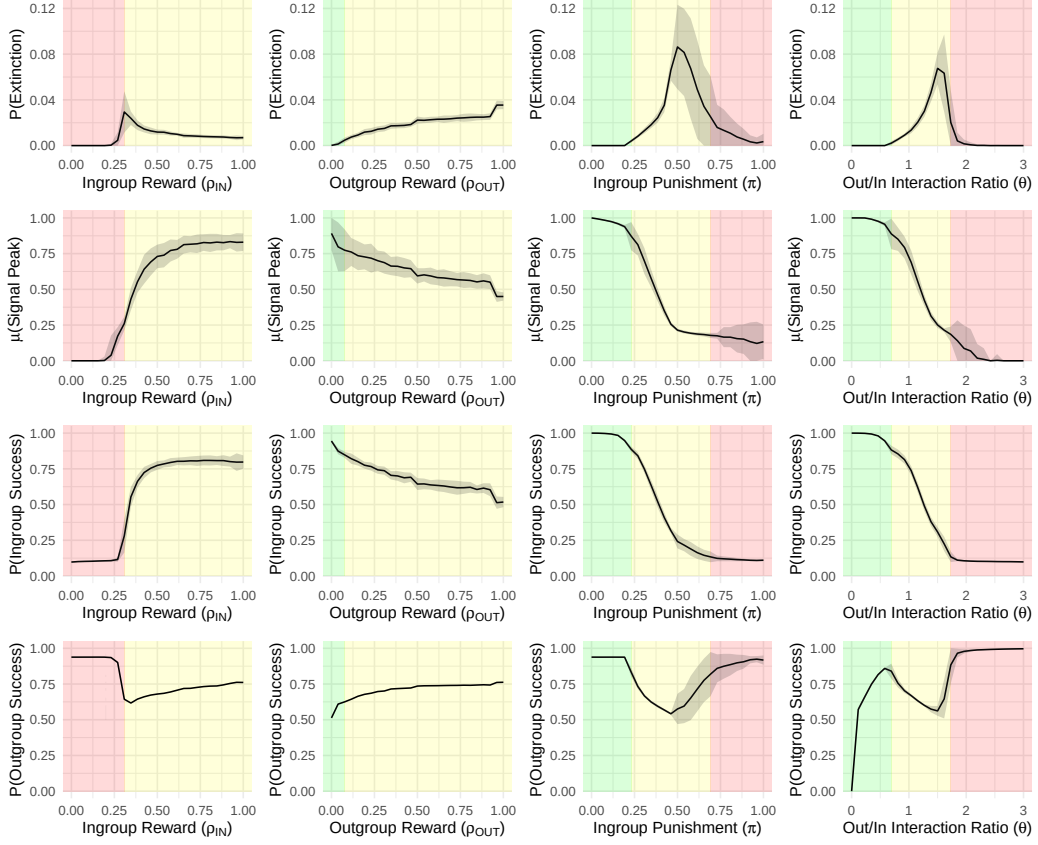
FIGURE 4. Sweeps of theoretically significant parameters holding all others constant. Each plot shows the relationship between a parameter and a feature of model dynamics. 95% confidence intervals are demarcated by the shaded gray band on either side of the line. Dynamic classes are shown by the shaded rectangles: green, saturation; yellow, cycling; red, suppression. Each column corresponds to 1 of the 4 parameters of interest. The x -axes show the parameters by which they differ: ingroup reward ( \rho_{IN} ), outgroup reward ( \rho_{OUT} ), ingroup punishment ( \pi ), and outgroup/ingroup interaction ratio ( \theta ). Rows correspond to four outcome features. Top: P(Extinction), the probability that a signal goes extinct and restarts, corresponding to the period of the cycles. Upper Middle: \mu (Signal Peak), the average knowledge of a signal among the ingroup, corresponding to the amplitude of the cycles. Lower Middle: P(Ingroup Success), the proportion of ingroup interactions which resulted in one or both of the ingroup agents recognizing their partner's signal and revealing their own identity. Bottom: P(Outgroup Success), the proportion of ingroup-outgroup interactions which resulted in the outgroup member identifying the ingroup member.
