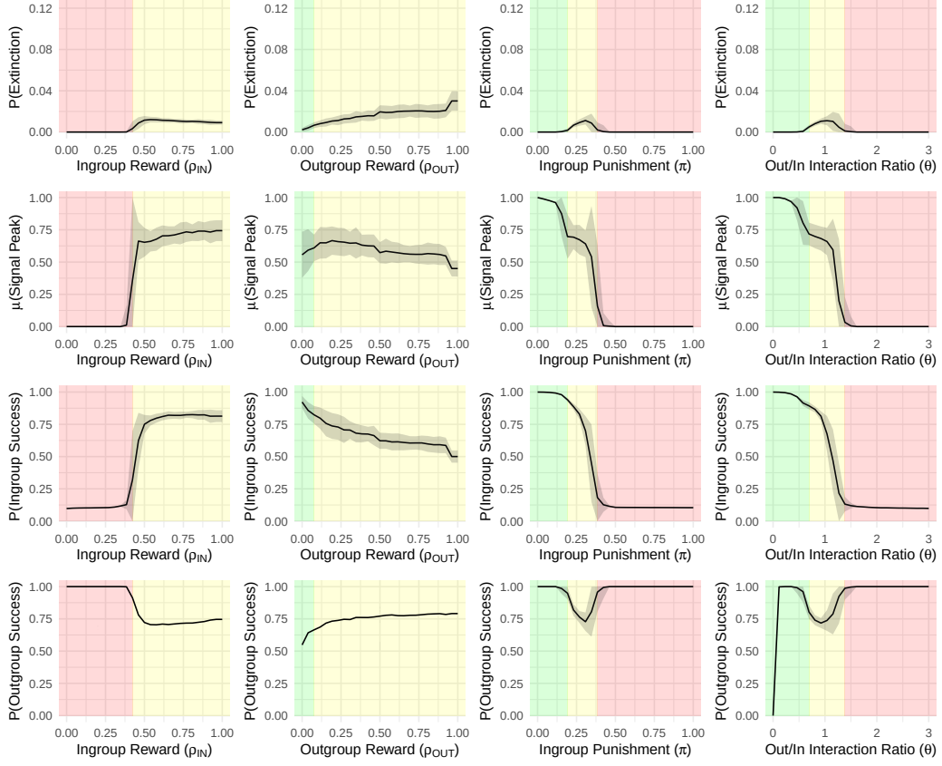
FIGURE D2. Sweeps of theoretically significant parameters holding all others constant as in Figure 4. Unlike Figure 4, which initializes with neutral conditions, wherein all ingroup signals are 0.1, these simulations initialize with suppression-like conditions, wherein all outgroup signals are 1. The patterns observed are similar to Figures 4 and D1, but differ notably due to artifacts of model design. First, P(\text{Extinction}) , or rate of cycling, is lower throughout the regions of parameter space that produce cycling. Second, the region of parameter space that produced cycling in companion plots has partly given way to suppression. The cause of both discrepancies is similar and stems from the mechanism for signal extinction and novel signal emergence. Both in a real system and our model the ingroup will develop a novel signals unable to use existing ones. However, in our model novel signals emerge only after reaching a prevalence threshold in the total population, here set to an average informational value of 0.15. In some cases, ingroup reward is not sufficient to overcome ingroup penalty at the interaction rate to reach that 0.15 threshold, and thus no signals can be renewed and the system remains in a state of suppression. Similarly, the rate of extinction is low even when cycling because it takes a substantial portion of the 1000 time steps to reach the threshold and enter cycling. However, these are both consequences of the model design and number of time steps; cycling is a stable attractor from this suppression-like state.
