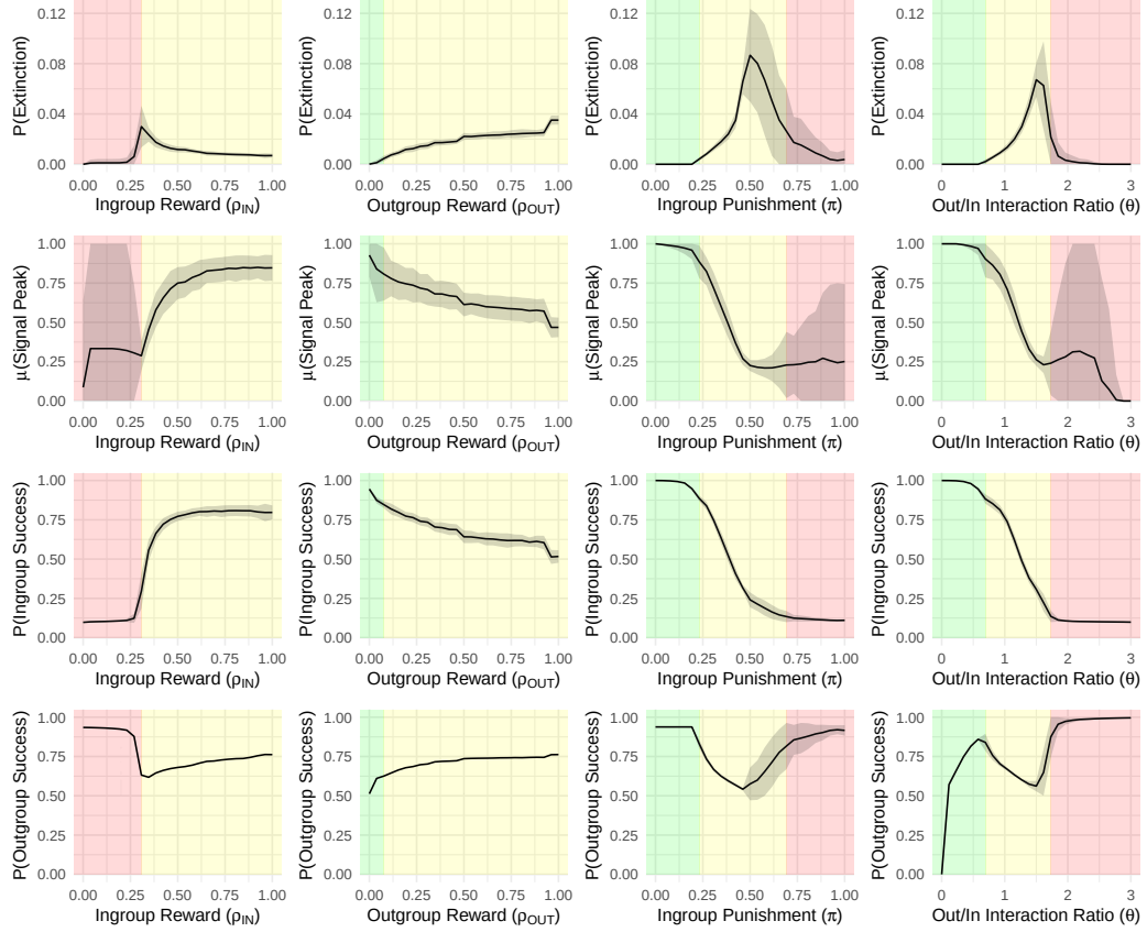
FIGURE D1. Sweeps of theoretically significant parameters holding all others constant as in Figure 4. Unlike Figure 4, which initializes with suppression-like conditions, wherein all ingroup signals are 0.1, these simulations initialize with saturation-like conditions, wherein all ingroup signals are 1. The patterns observed are nearly identical to Figure 4, differing only for the suppression regime for \mu(\text{Signal Peak}) . Here we observe a wide confidence interval indicating that sometimes 1000 time steps are sufficient to shift the signals away from 1, and sometimes they are not.
