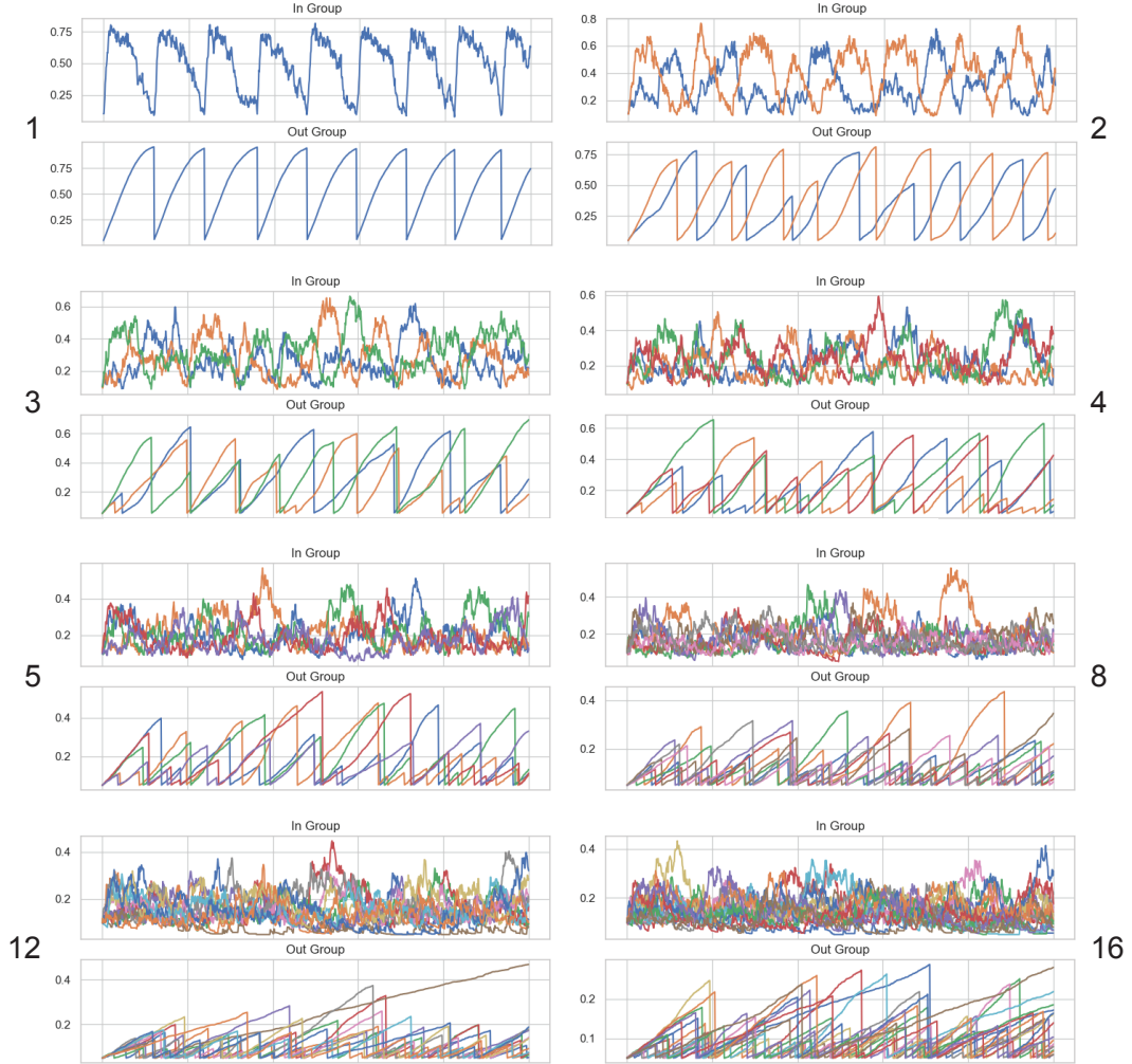
FIGURE B1. Signaling dynamics sweeping K . All other values set to the defaults given by Table 1
