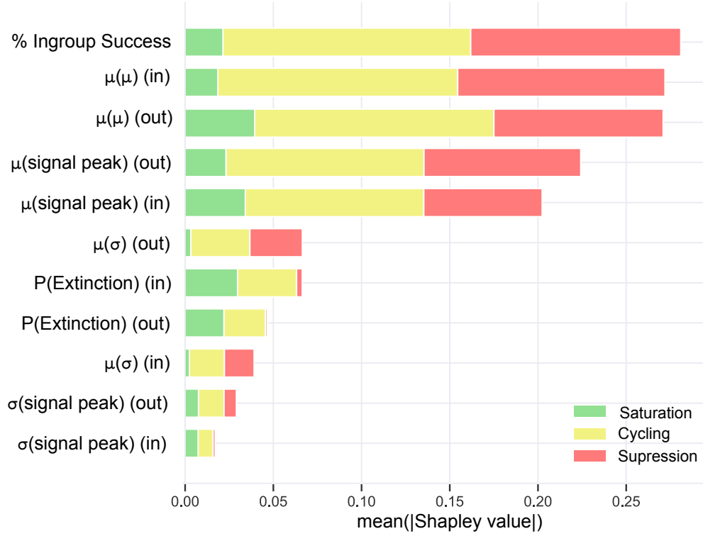
FIGURE C1. Shapley decomposition of the random forest model. Length of each bar shows the contribution of the feature to determining the probability of each class of model dynamics. A long bar in a particular color indicates that the feature is highly informative in determining whether it belongs to the class associated with that color. A short bar indicates that the feature is not very informative.
