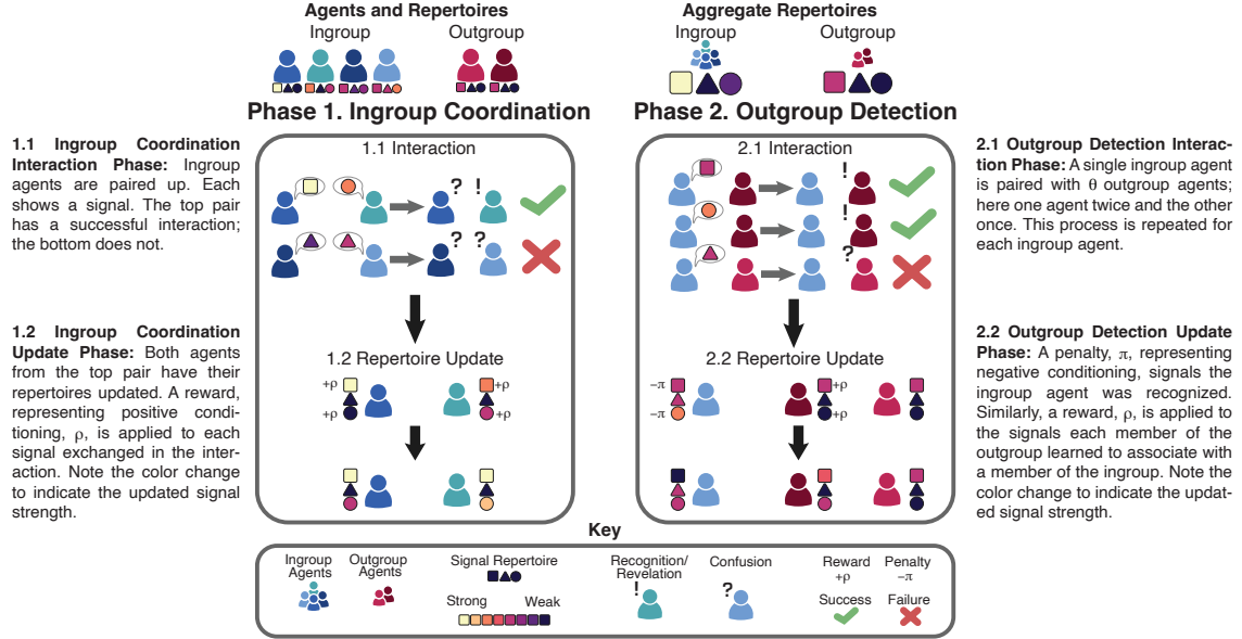
FIGURE 2. A schematic of the agent-based model representing a single time step. Signaling repertoires are denoted by the array of colored shapes. Each agent has its own signaling repertoire, distinguished by the different colors for each shape, indicating the informational value of each signal for that particular agent at that time. Stronger signals are lighter, weaker are darker. Aggregate signaling repertoires, the primary outcome of the model, are also pictured, representing informational values averaged across all agents. Not pictured is the extinction/emergence phase where signals that have risen and then fallen to particular thresholds in the ingroup population are reset to their initial values in the ingroup and outgroup. This represents the emergence of a novel signal at the location in the signal repertoires that was occupied by a newly extinct signal.
